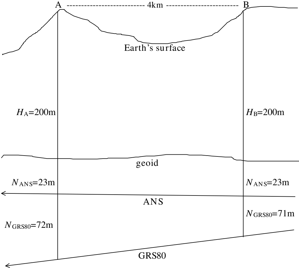
FIGURE 2 A measured terrain distance of 4km and typical station heights in relation to the geoid ( H ), Australian National Spheroid ( h_{ANS} = H + N_{ANS} ) and the Geodetic Reference System 1980 ( h_{GRS80} = H + N_{GRS80} ) spheroid.
